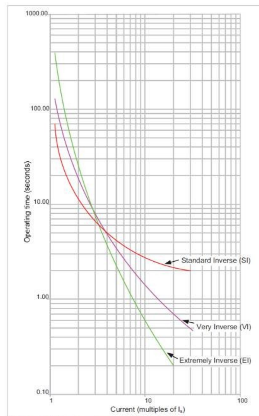
IEC 60255 IDMT relay characteristics; TMS=1.0
